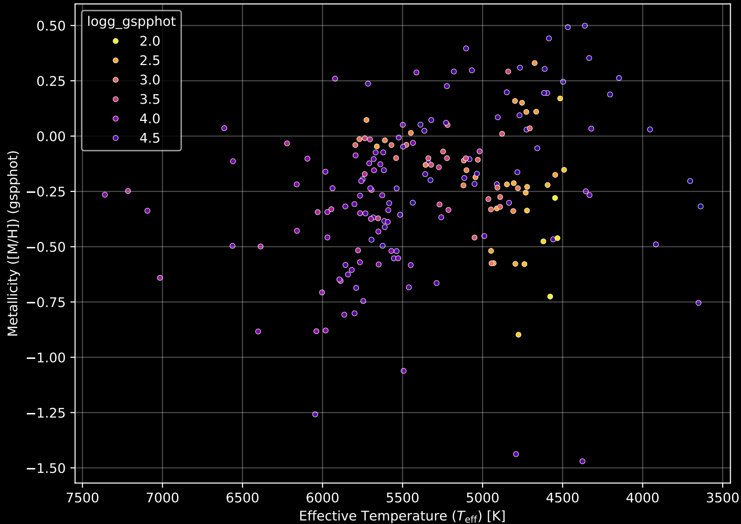
APOGEE DR17 Field: [242+44_MGA] Stellar Population Parameters (n= 193)
