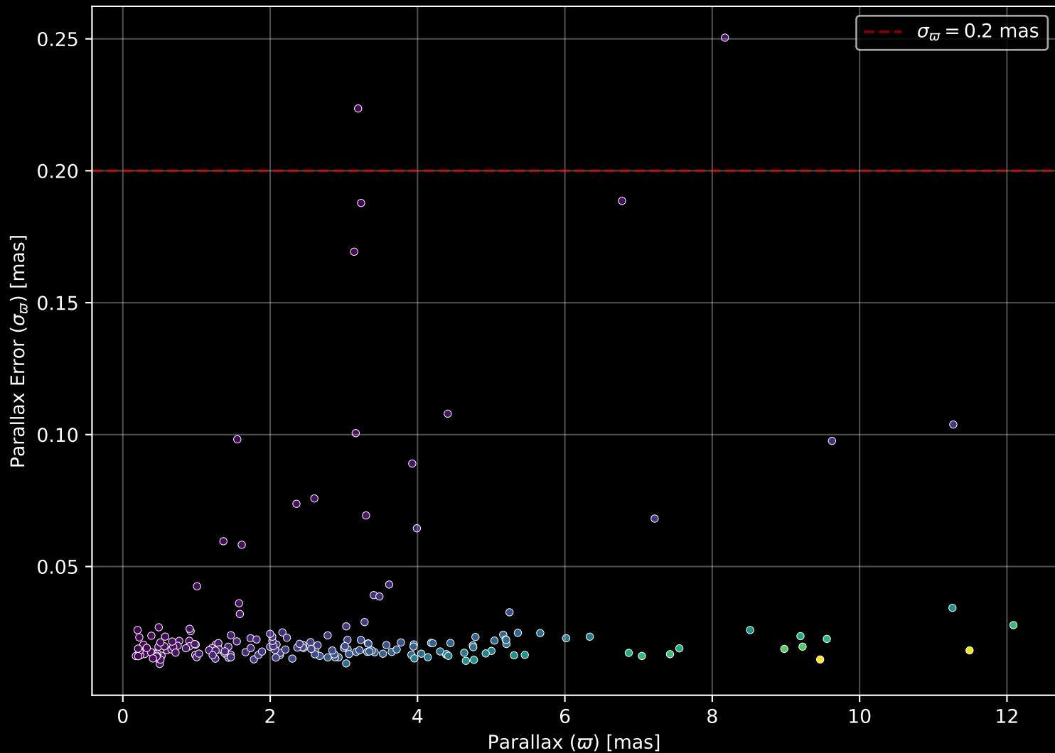
APOGEE DR17 Field: [242+44_MGA] Parallax Quality (n= 193)
